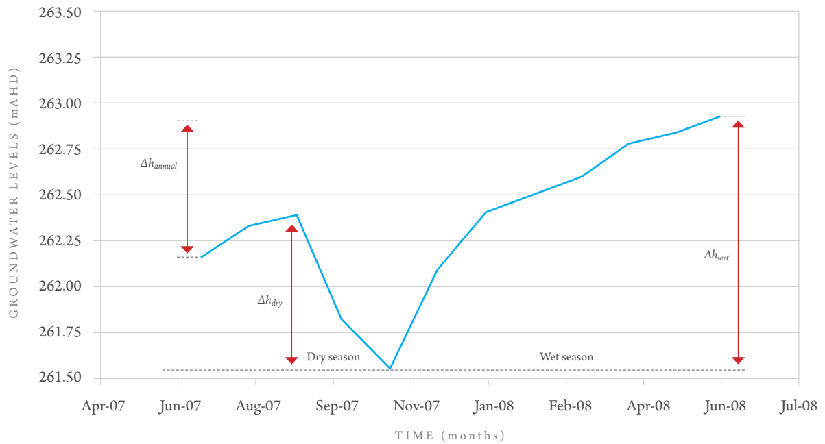
FIGURE 5: Monthly average groundwater levels
